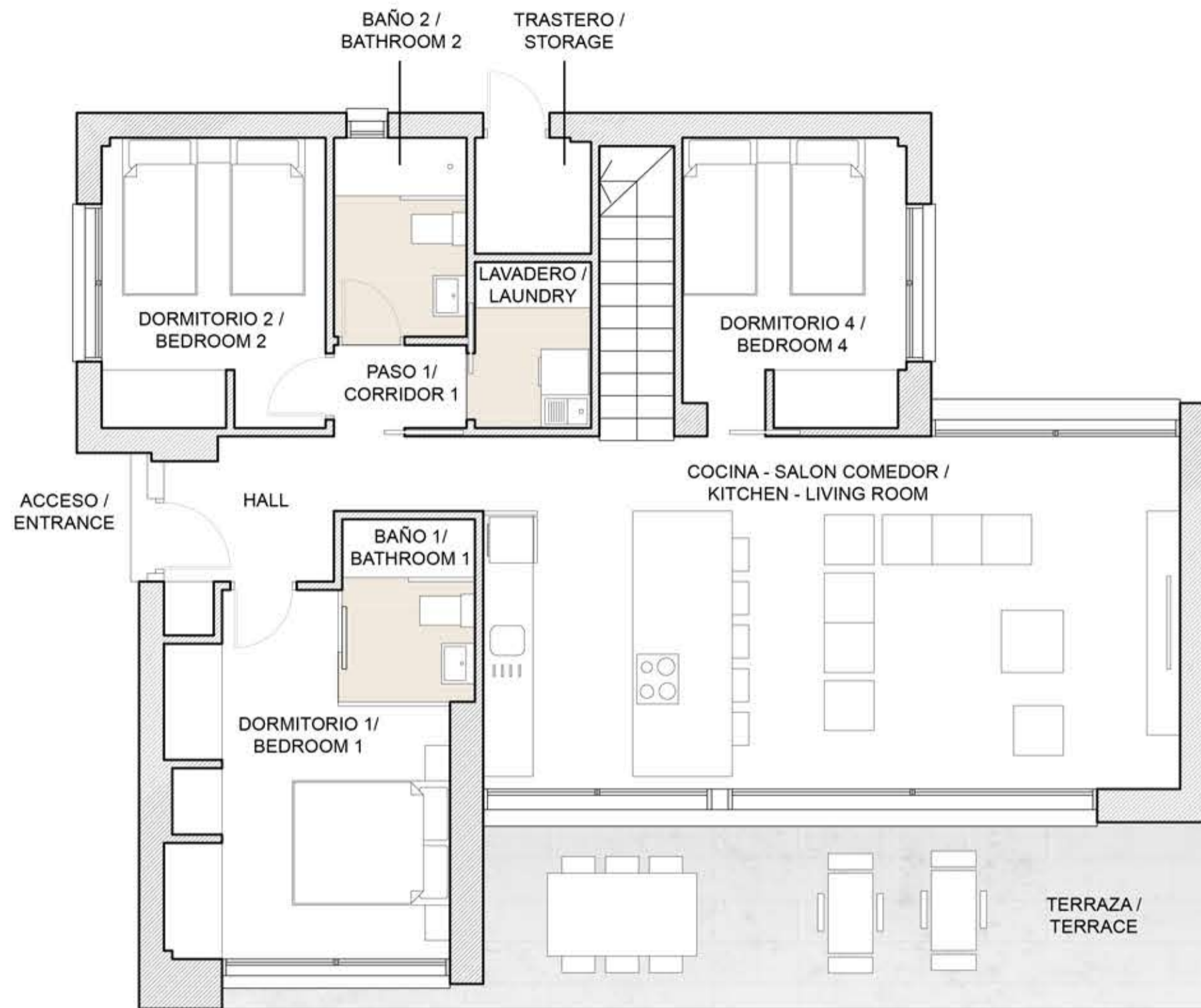
PLANTA BAJA / GROUND FLOOR
